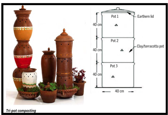
TRI-POT COMPOSTING
