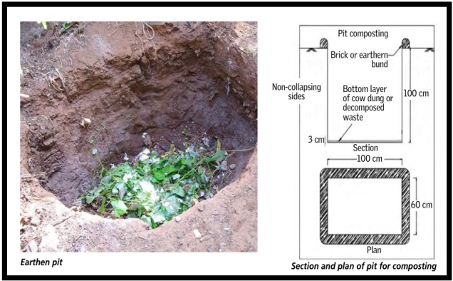
PIT COMPOSTING
