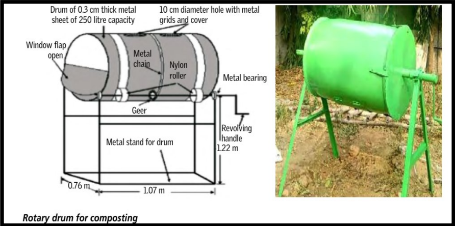
ROTARY DRUM COMPOSTING
