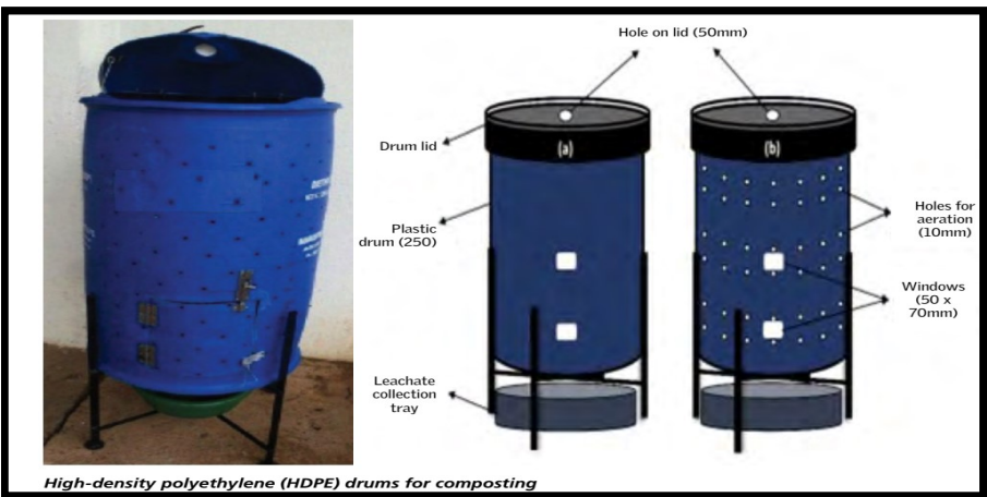
DRUM COMPOSTING
