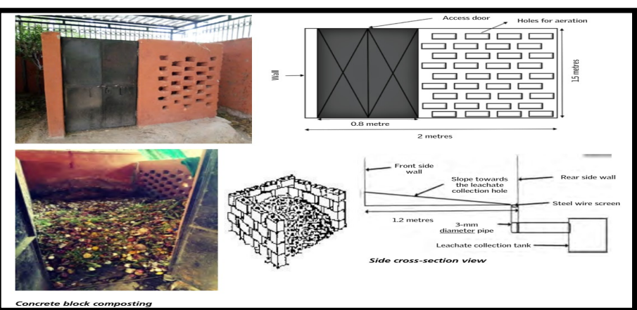
CONCRETE BLOCK COMPOSTING
