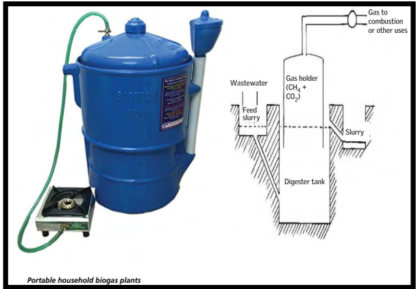
PORTABLE BIOGAS PLANT
