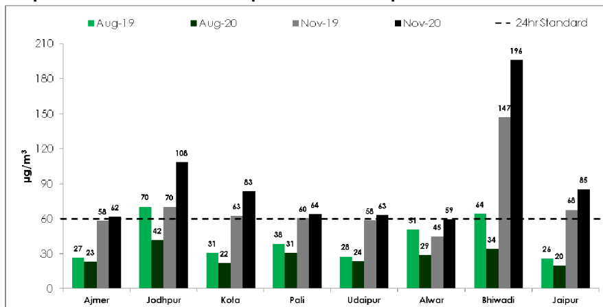
Graph 2: Difference in winter pollution build-up: 2020 winter vs 2019 winter (monthly averages)
