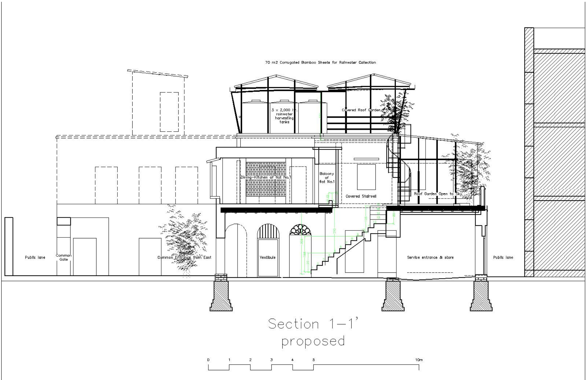
Bamboo and mud guest rooms with Rain Water Harvesting in North Kolkata by Laurent Fournier
